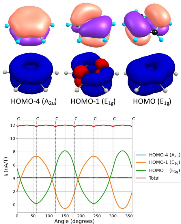
Fig. 2 The \pi orbitals of benzene (top), their MIRC (middle) and the dependence of their contributions to the MIRC strength (in nA/T) as a function of the angle of the integration plane (bottom). The orbital pictures are made with ParaView. 87
