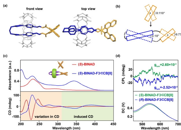
Fig. 3 Structural and chiroptical analysis of the ring-in-ring complex. (a) Crystal structure of (S)-BINAD-F3 ⊂ CB[8] ( CB[8] in gray; F3 moiety in blue; and BINAD moiety in orange. Hydrogen atoms, counterions, and solvents are omitted for clarity). (b) Illustration of the structural chirality induced by the attachment to an axial chiral moiety. (c) UV-vis and CD spectra for (S)-BINAD and (S)-BINAD-F3 ⊂ CB[8] . Similar spectra for (R) -enantiomers exhibit the same profiles, except for inverted signal signs in CD spectra (Fig. S35†). (d) CPL spectra and g_{\text{lum}} measured for both (S) - and (R)-BINAD-F3 ⊂ CB[8] (conditions: \text{H}_2\text{O} , 100 \mu\text{M} , 25 °C, \lambda_{\text{ex}} = 350 nm).
