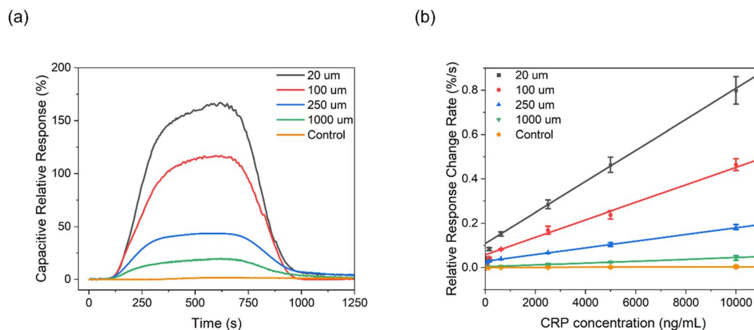
Fig. 4 (a) Representative capacitive sensograms of the anti-CRP modified PANI interface in response to 10.0 \mu\text{g mL}^{-1} CRP within varying microfluidic channel heights and under a flow rate of 10 \mu\text{L min}^{-1} . (b) Capacitive dose–response curves derived from the 15 seconds of temporal data during the association regime. C_r was normalized relative to baseline before each injection. The control (orange) sampling represents that from PANI electrodes without anti-CRP modification, measured within a 1000 \mu\text{m} channel. Error bars represent the standard deviation across three individual electrodes ( n = 3 ).
