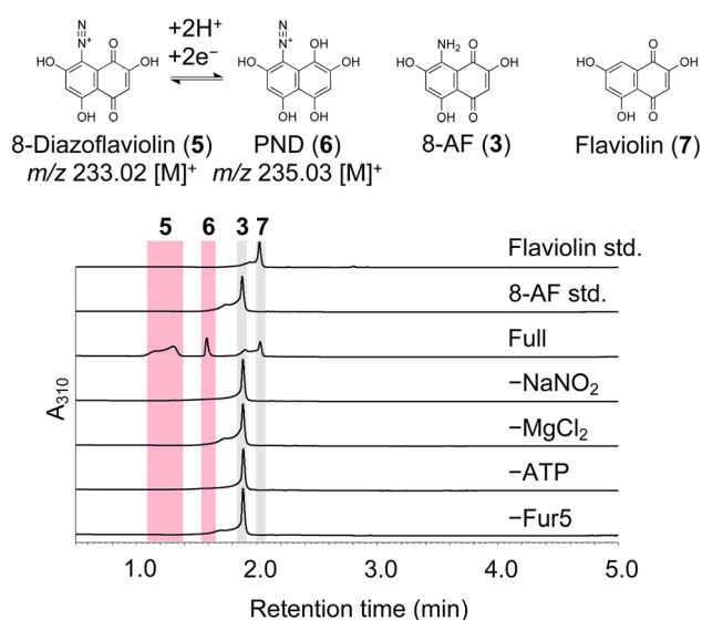
Fig. 3 In vitro assays of the enzymatic activity of Fur5. HPLC-UV/VIS analysis of the Fur5 reaction mixture. The assay conditions are described in the ESI.† A_{310} , absorbance at 310 nm.
