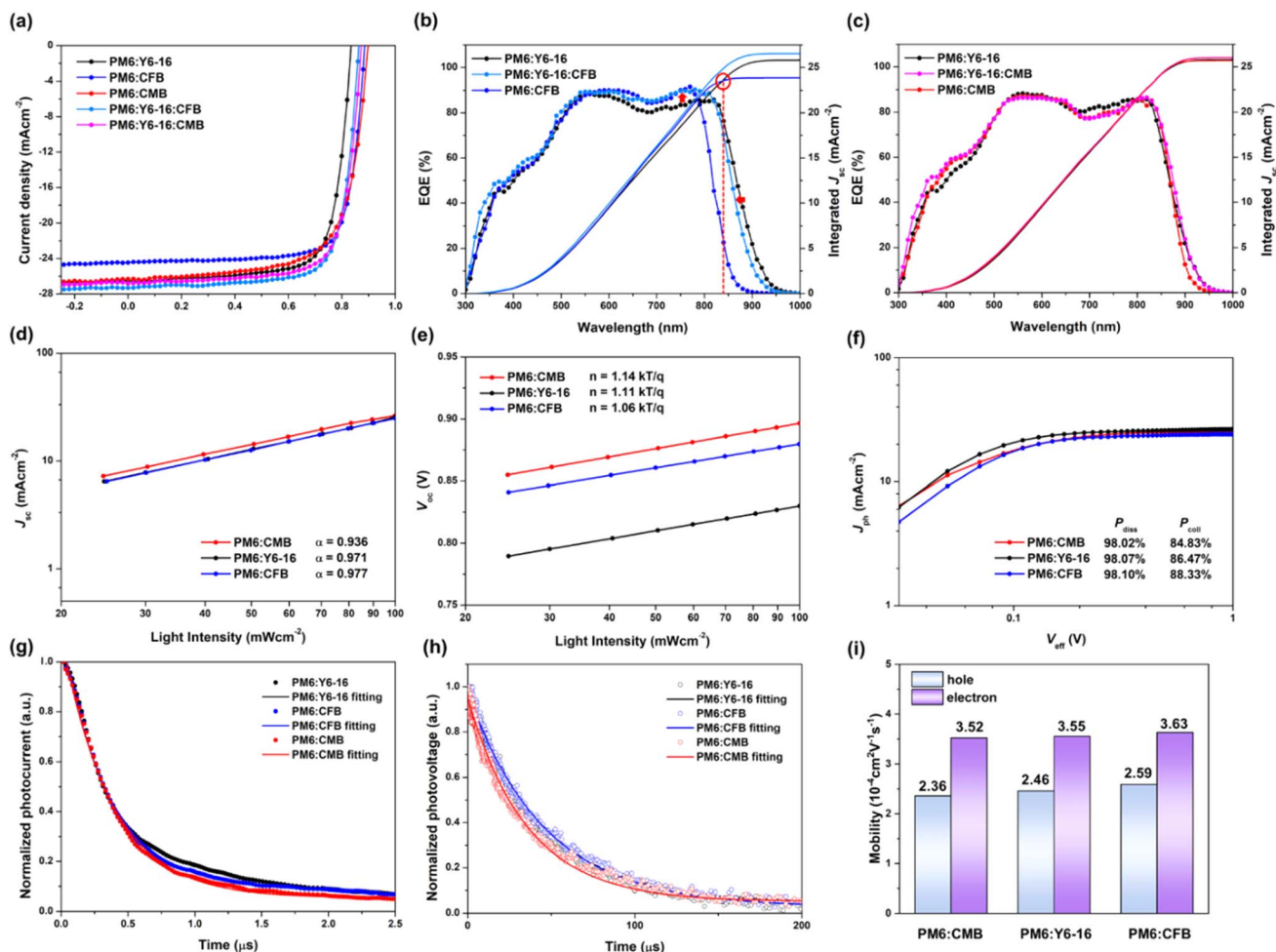
Fig. 4 (a) J-V curves of PM6:Y6-16, PM6:CFB, PM6:CMB, PM6:Y6-16:CFB and PM6:Y6-16:CMB devices. EQE spectrum of (b) CFB-based devices and (c) CMB-based devices. (d) J_{sc} versus light intensity, (e) V_{oc} versus light intensity and (f) J_{ph} versus V_{eff} spectra for the PM6:CMB, PM6:Y6-16 and PM6:CFB devices. (g) Transient photocurrent curves (dots) and corresponding fitting curves (solid lines) and (h) transient photovoltage curves (circles) and corresponding fitting curves (solid lines) for the optimized binary devices. (i) SCLC electron and hole mobilities of the optimized binary devices.
