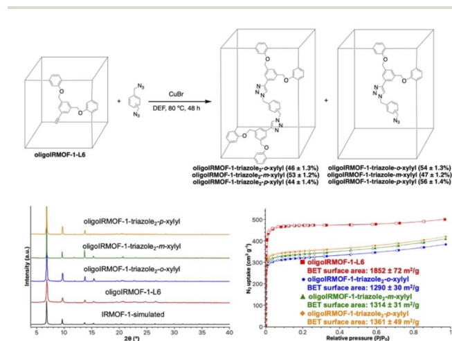
Fig. 7 (Top) PSM of oligoIRMOF-1-L6 with diazido xylyl isomers. The contents of each compound in this PSM reaction were determined by solution 1 H NMR of the digested reaction products. (Bottom left) PXRD patterns of simulated IRMOF-1 (black), oligoIRMOF-1-L6 (red), oligoIRMOF-1-triazole 2 - o -xylyl (blue), oligoIRMOF-1-triazole 2 - m -xylyl (green), oligoIRMOF-1-triazole 2 - p -xylyl (orange). (Bottom right) Nitrogen isotherm of oligoIRMOF-1-L6 (red squares), oligoIRMOF-1-triazole 2 - o -xylyl (blue circles), oligoIRMOF-1-triazole 2 - m -xylyl (green triangles), oligoIRMOF-1-triazole 2 - p -xylyl (orange diamonds). The filled and unfilled squares correspond to adsorption and desorption, respectively.
