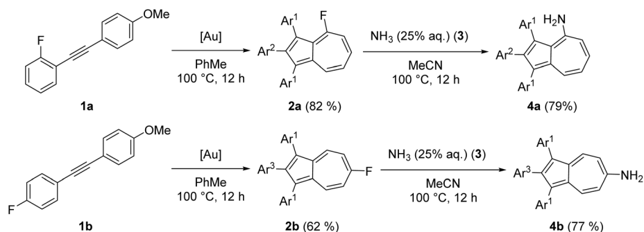
Scheme 1 Synthesis of amino-substituted azulenes 4a-b from the azulenes 2a-b , the latter deriving from the dimerization push-pull diyne 1a or 1b . Conditions: 1a-b (1.00 eq.) [IPr*Au(NCMe)]SbF 6 (5 mol%), PhMe, 100 °C, 12 h; 2a-b (1.00 eq.), 3 (50 eq., 25% aq.), MeCN, 100 °C, 12 h. Ar 1 = para -methoxyphenyl-, Ar 2 = ortho -fluorophenyl-, Ar 3 = para -fluorophenyl-.
