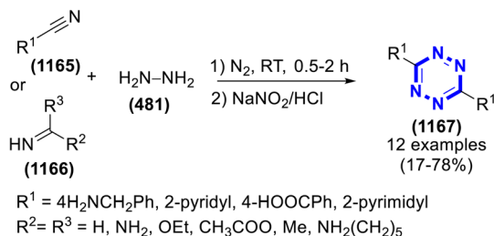
Scheme 323 Synthesis of 1,2,4,5-tetrazines under catalyst-free conditions.
