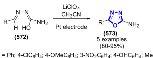
Scheme 153 Synthesis of oxadiazole frameworks catalyzed by \text{LiClO}_4 via an electrolysis method.
