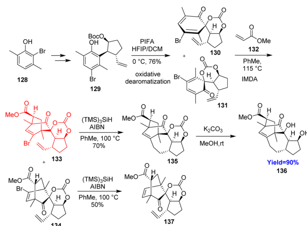
Scheme 17 Synthesis of tetracyclic core of calyciphylline N ( 136 ). 49
