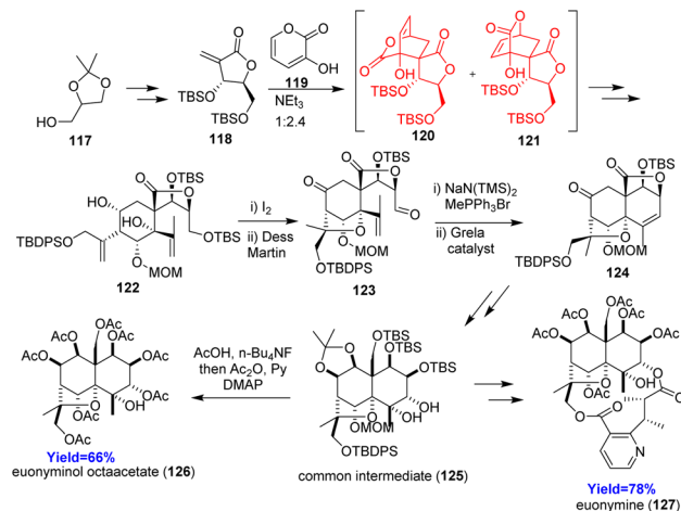
Scheme 16 Total synthesis of euonymine ( 127 ) and euonyminol octaacetate ( 126 ). 48
