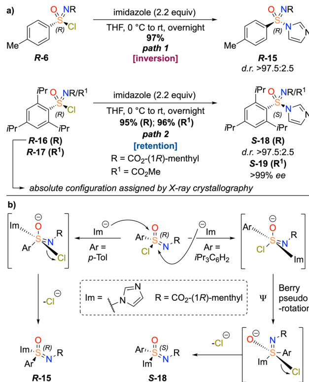
Scheme 4 (a) Synthesis of enantioenriched sulfonimidoyl imidazoles R - 15 , S - 18 , and S - 19 via inversion or retention of the sulfur stereocentre; (b) proposed substitution mechanism to account for observed retention of stereochemistry.
