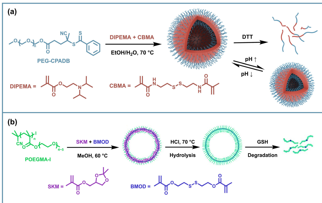
Fig. 1 Schematic illustration of disulfide-based stimulus-responsive disassembly of PISA NPs: (a) reductant-responsive vesicles based on PEG- b -P(DIPEMA-co-CBMA). (b) Reductant-responsive vesicles based on POEGMA- b -P(SK-co-BMOD). Adapted with permission from ref. 63. Copyright 2021 The Royal Society of Chemistry.
