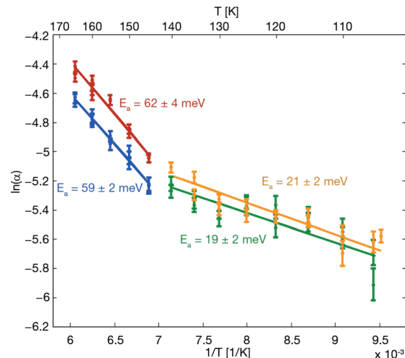
Fig. 11 The Arrhenius plot from temperature-dependent measurements of C 4 H 4 S dynamics on Cu(111), taken at 0.7 Å -1 along the \overline{\Gamma K} -azimuth, reveals two competing activated processes. The gradient gives an apparent activation barrier for rotation of 19 \pm 2 meV at 0.015 ML (green) and 21 \pm 2 meV at 0.022 ML (orange), while jump diffusion is more strongly activated with E_a = 59 \pm 2 meV at 0.015 ML (blue) and E_a = 62 \pm 4 meV at 0.022 ML (red). (Reprinted with permission from ref. 66, Copyright 2013 by the American Chemical Society).
