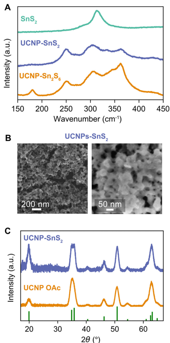
Fig. 5 Annealing Sn 2 S 6 4- -capped 9-nm NaYF 4 : 8% Tm 3+ UCNP onto a UCNP-SnS 2 nanocomposite. (A) Raman spectra of the Sn 2 S 6 4- -capped UCNP before (orange line) and after (blue line) annealing. Also shown is the spectrum of the SnS 2 matrix formed by annealing Na 4 Sn 2 S 6 (green line). (B) SEM images of the UCNP embedded in the SnS 2 matrix. (C) X-ray diffraction spectra of the UCNP-SnS 2 nanocomposite (blue line) and oleate-capped UCNP (orange line). The reference spectrum for hexagonal-phase NaYF 4 (PDF# 04-022-5333) is also shown (green line).
