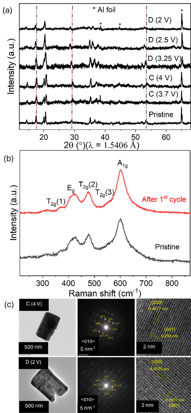
Fig. 6 (a) Ex situ XRD patterns of LMO2 at different states of charge. (b) Comparative Raman spectra of LMO2 in pristine and after the 1 st cycle. (c) Ex situ TEM, SAED and HRTEM analysis of the LMO2 cathode charged to 4 V (top) and discharged to 2 V (bottom). The (010) zone axis was taken for the SAED patterns.
