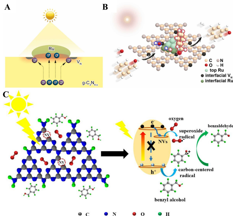
Fig. 13 Schematic diagrams of A: photoinduced charge transfer/separation at the Ru/g-C_3N_{4-x} interface and B: photocatalytic mechanism of H_2 evolution coupled with selective benzyl-alcohol oxidation over the Ru/g-C_3N_{4-x} catalyst. Reproduced with permission from ref. 134. C: proposed mechanisms of the photocatalytic selective oxidation of BA to BAD over N-deficient g-C_3N_4 . Reproduced with permission from ref. 109.
