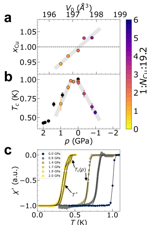
Fig. 2 Dependence of physical properties on chemical and hydrostatic pressure in LaCuSb 2 . (a) Refined copper occupancy x_{Cu} derived from single-crystal XRD, versus room-temperature unit cell volume V_0 = ca^2 derived from powder XRD. (b) Superconducting dome derived from magnetization measurements, showing the measured midpoint T_c versus V_0 at ambient pressure, along with measured midpoint T_c versus hydrostatic pressure p for the optimized sample (black), the latter of which has refined occupancy x_{Cu} = 0.988(5) . Solid grey lines are fits to the data with linear trendlines. (c) Real part of the AC susceptibility for LaCuSb 2 under hydrostatic pressure. The transition T_c is seen to decrease and there appears to be a double-peak feature near T_c(p) and T^* \approx 0.35 K at higher pressures. Solid lines are fits to the data using eqn (S4) (ESI†).
