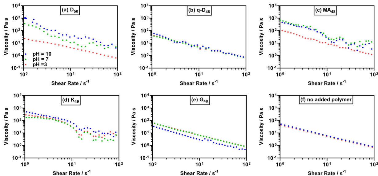
Fig. 4 Viscosity vs. shear rate for 50% w/w IOP suspensions with 0.5% w/w (a) D 50 , (b) q-D 48 , (c) MA 48 , (d) K 49 , (e) G 48 , and (f) without added polymer at pH = 3 (red dots), pH = 7 (green dots) and pH = 10 (blue dots). The 0.5% w/w polymer additive concentration is based on IOP concentration.
