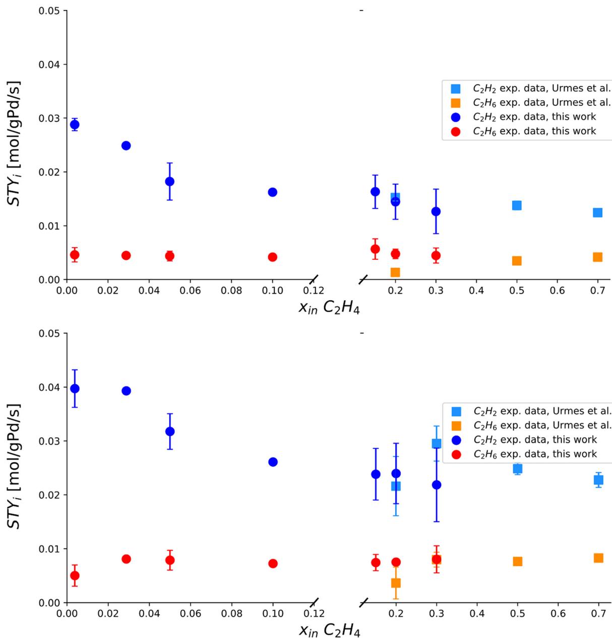
Fig. 4 Experimentally measured space-time yields of C_2H_2 and C_2H_6 ( STY_{C_2H_2} [ \text{mol g}_{\text{Pd}}^{-1} \text{s}^{-1} ] and STY_{C_2H_6} [ \text{mol g}_{\text{Pd}}^{-1} \text{s}^{-1} ]) plotted against the inlet molar fraction of C_2H_4 . Top) Trend obtained at 323 K, i.e. 50 °C. Bottom) Trends obtained at 333 K, i.e. 60 °C. The x -axis is reported with a broken plot representation to precisely quantify the behavior across the composition range investigated. Includes experimental data by Urmès et al. and experimental data from this work. The standard deviation of experimental measurements is reported through error bars for points whose reproducibility has been verified through at least two repeated experiments.
