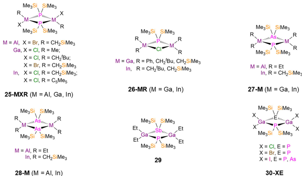
Fig. 7 Dimeric group 13 P'' complexes [M(R)(X)(μ-P'')] 2 ( 25-MXR : M = Al, Ga, In; X = Cl, Br; R = Me, CH 2 t Bu, CH 2 SiMe 3 , η 1 -Cp*, Cp* = C 5 Me 5 ), [(M(R)) 2 (μ-P'')(μ-Cl)] ( 26-MR : M = Ga, In; R = Ph, CH 2 t Bu, CH 2 SiMe 3 ), [(M(R)) 2 (μ-P'')(μ-As'')] ( 27-M : M = Al, R = Et, M = In, R = CH 2 SiMe 3 ), [(M(R)) 2 (μ-As'')] ( 28-M : M = Al, R = Et, M = In, R = CH 2 SiMe 3 ), [(Ga(Et)) 2 (μ-P'')(μ-Sb'')] ( 29 ), [(Ga(X)) 2 (μ-P'')(μ-E(SiMe 3 ) 2 )] ( 30-ClP : X = Cl, Pn'' = P''; 30-BrP : X = Br, Pn'' = P''; 30-IP : X = I, Pn'' = P''; 30-IAs : X = I, Pn'' = As'').
