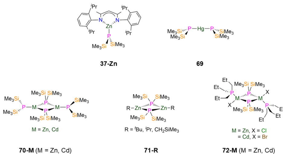
Fig. 20 Monomeric and dimeric group 12 P'' complexes [Zn(DiPPNacnac)(P'')] ( 37-Zn ; DiPPNacnac = CH((CH_3)_2CN(Dipp))_2 ; Dipp = C_6H_3iPr_2\text{-}2,6 ), [Hg(P'')]_2 ( 69 ), [M(P'')(\mu\text{-}P'')]_2 ( 70-M , M = Zn, Cd ), [Zn(R)(\mu\text{-}P'')]_2 ( 71-R , R = tBu, iPr, CH_2SiMe_3 ), [M(P''Pr_3)(X)(\mu\text{-}P'')]_2 ( 72-Zn : M = Zn, X = Cl ; 72-Cd : M = Cd, X = Br ).
