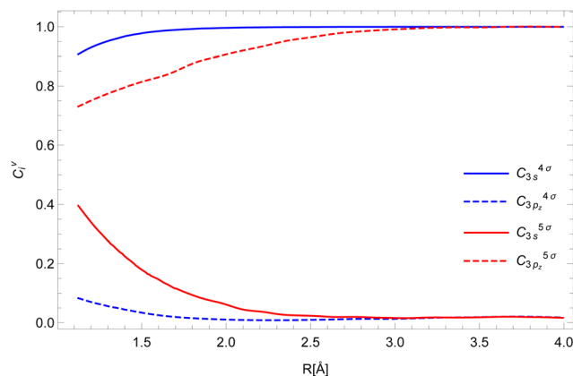
Fig. 3 The expansion coefficients C_v^i of the valence shell v into atomic orbitals i for the 4\sigma (blue) and 5\sigma (red) orbitals.
