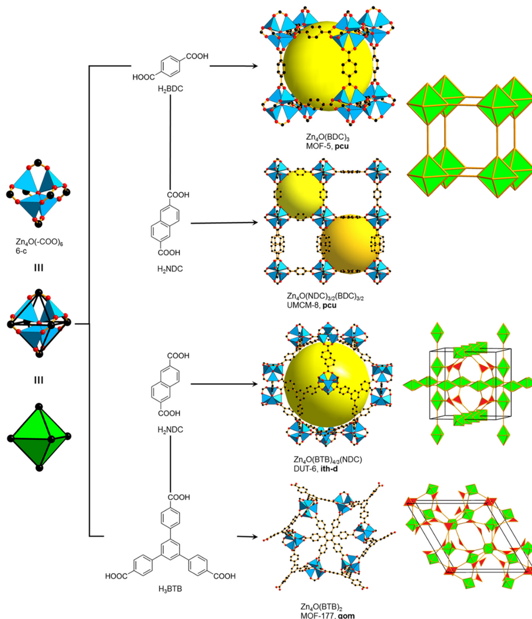
Fig. 3 MOFs constructed from Zn 4 O(-COO) 6 SBUs. Color code: black, C; red, O; blue polyhedra, Zn. The yellow spheres represent the empty space in the framework. Hydrogen atoms are omitted for clarity. Adapted from ref. 30. Copyright 2024 Springer Nature.
