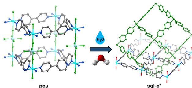
Fig. 1 Illustration showing the phase transition of a prototypical pcu topology HUM to an sql-c* topology CN, in the presence of excess water.
