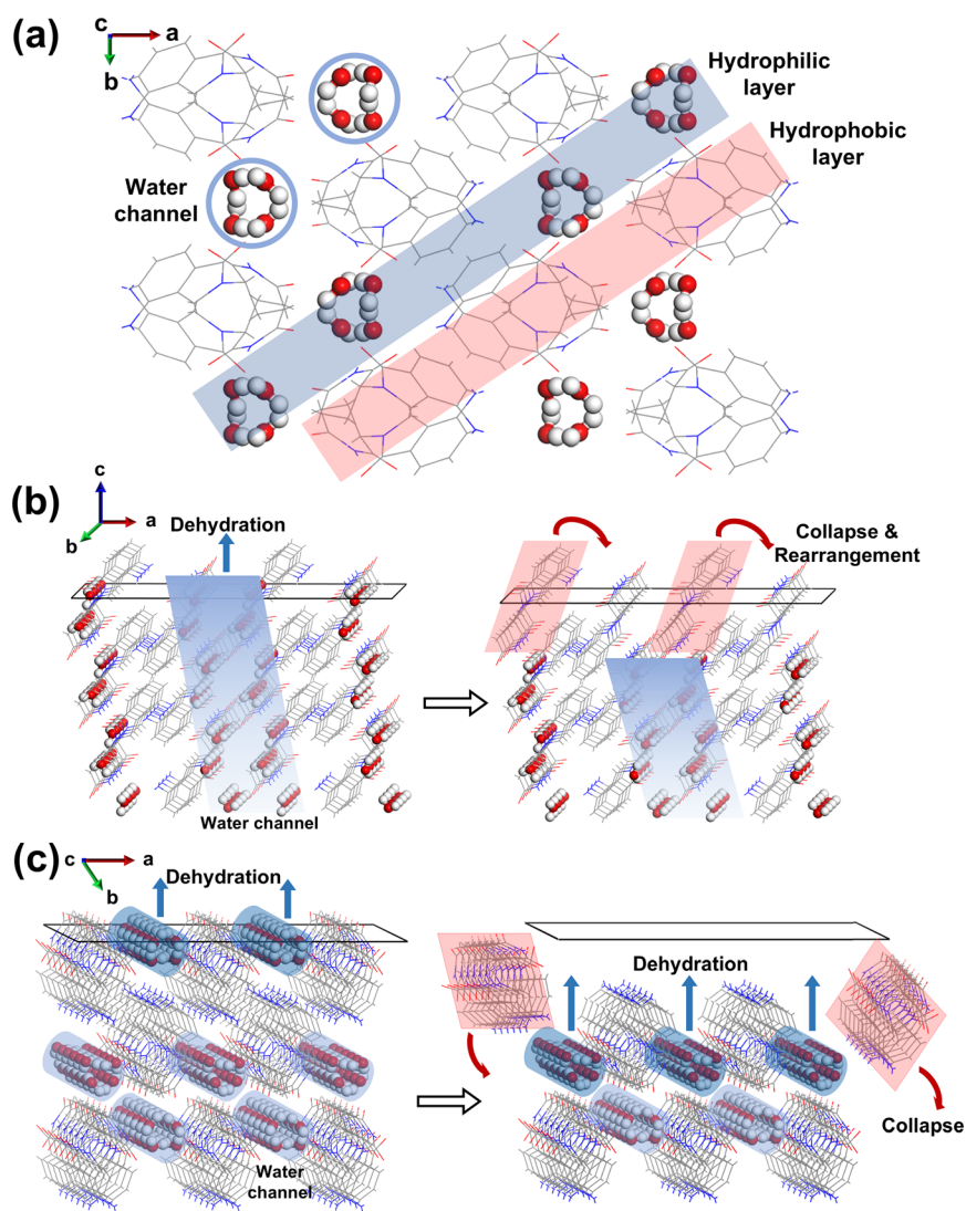
Fig. 5 (a) Supercell structures along the c -axis of crystals E1 and E2. Schematic diagrams of dehydration channel changes during the dehydration process (b) on E1 crystal face (0\ 0\ 1) and (c) on E2 crystal face (1\ 0\ 0) .
