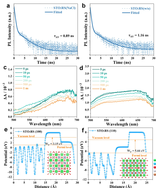
Fig. 3 TRPL decay curves of (a) STO:RS(NaCl) and (b) STO:RS(w/o) measured at 440 nm. TAS of (c) STO:RS(NaCl) and (d) STO:RS(w/o). Theoretical calculated work functions of the (e) {100} and (f) {110} facets of STO:RS(NaCl).
