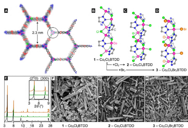
Fig. 1 (A) Schematic presentation of the structure of the Co(II) MOF Co 2 Cl 2 BTDD, (B)–(D) NPD structures of the SBU and local coordination environments of the Co metal centers Co 2 Cl 2 BTDD, Co 2 Cl 4 BTDD, and Co 2 Cl 2 Br 2 BTDD, respectively, and (E) PXRD data and (F)–(H) SEM images of Co(II) MOF before and after Br 2 and Cl 2 adsorption. Reproduced with permission from ref. 22. Copyright 2017, American Chemical Society.
