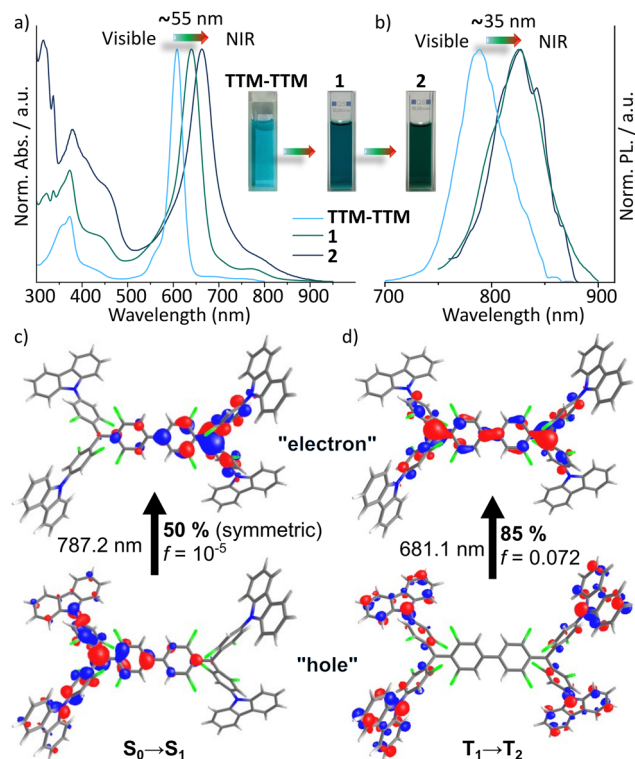
Fig. 3 (a) UV-Vis absorption spectra and photographs taken at ambient light. (b) Photoluminescence spectra in toluene solutions of TTM-TTM , 1 , and 2 . Natural transition orbitals (NTOs) with hole (h + ) and electron (e - ) for (c) the singlet and (d) the triplet state lowest energy transitions of 2 (in their optimized ground state geometry).
