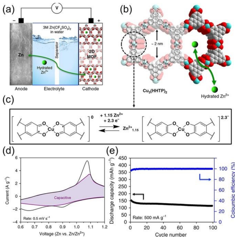
Fig. 10 Shows how \text{Cu}_3(\text{HHTP})_2 performs electrochemically as a cathode for rechargeable ZIBs. a) Zn- \text{Cu}_3(\text{HHTP})_2 cell schematic depiction. b) The \text{Cu}_3(\text{HHTP})_2 chemical structure. c) The anticipated redox mechanism in the \text{Cu}_3 coordination unit ( \text{HHTP})_2 . d) CV profile at 0.5 \text{ mVs}^{-1} @1, together with the capacitive contribution (shaded region). e) Cycling efficiency at 500 \text{ mA g}^{-1} @1 [157].
