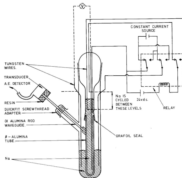
Fig. 3 Apparatus for AE sensing in high-temperature Na-S batteries. Reproduced with permission from ref. 46 . Copyright 1978, Springer Science.
