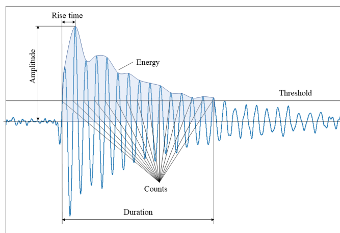
Fig. 2 Features of typical AE waveform
