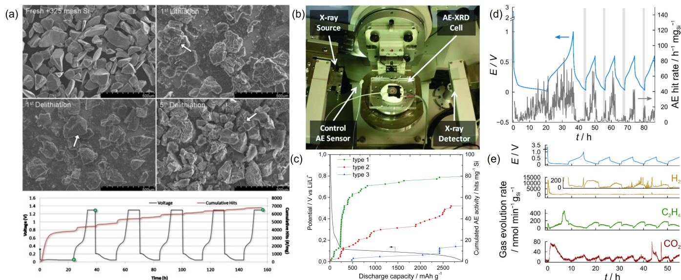
Fig. 6 (a) SEM images and voltage-cumulative hits-time diagram of Si electrodes. Reproduced with permission from ref. 21 . Copyright 2010, The Electrochemical Society. (b) Setup for operando XRD-AE experiments. Reproduced with permission from ref. 33 . Copyright 2011, AIP Publishing. (c) Evolution of electrode potential and cumulated AE activity as a function of discharge capacity. Reproduced with permission from ref. 35 . Copyright 2015, Elsevier. (d) Voltage-AE hit rate diagram of a Si/C composite electrode. (e) Gas evolution results of a Si/C composite electrode. Reproduced with permission from ref. 23 . Copyright 2018, American Chemical Society.
