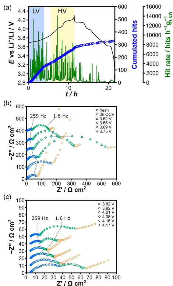
Fig. 9 (a) Voltage profile of the initial cycle of an LNO half-cell. (b) Low-voltage and (c) high-voltage regions Nyquist plots of the EIS data. Reproduced with permission from ref. 19 . Copyright 2020, Wiley-VCH.
