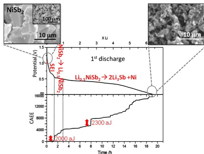
Fig. 7 Voltage profile and cumulated AE energy of NiSb 2 /Li cell as functions of time. Reproduced with permission from ref. 31 . Copyright 2010, Elsevier.
