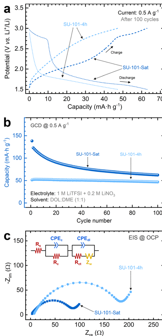
Fig. 4 (a) Galvanostatic charge–discharge curves of the SU-101-4h and SU-101-Sat cathodes after cycling at a C/2 rate ( 0.5 \text{ A g}^{-1} ) between 1.5 and 3.0 V vs. Li + /Li + . Charge profiles are depicted with dashed lines, while discharge profiles are depicted with dotted lines. Arrows indicate the charge and discharge directions. (b) Capacity decay tests of SU-101-4h and SU-101-Sat cathodes for 100 cycles. Each sphere represents the capacity measured from one charge–discharge cycle. (c) Nyquist plots after cycling performance tests measured at the open circuit potential (OCP). The inset depicts the equivalent circuit model used to fit Nyquist plots.
