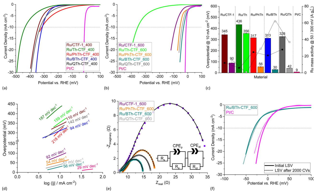
Fig. 8 HER LSV polarization curves in 0.5 \text{ mol L}^{-1} \text{H}_2\text{SO}_4 of (a) Ru/CTF_400 and (b) Ru/CTF_600. (c) Overpotentials (left bars for _400, right bars for _600 samples), Ru mass activities (filled boxes @ 300 mV, empty boxes @ 50 mV) and (d) Tafel plots of Ru/CTFs. (e) Nyquist plots at -100 \text{ mV} vs. RHE and fitted EEC models (solid lines) of Ru/CTF_600 with resistors for the electrolyte resistance, R_s , the electrode porosity, R_p , and the charge transfer, R_{ct} , as well as constant phase elements assigned to the electrode porosity, \text{CPE}_p , and double layer capacitance, \text{CPE}_{dl} . 109–111 (f) LSV polarization curves of Ru/BTh-CTF_600 after 2000 CV cycles durability test.
