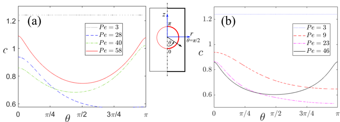
Fig. 6 Variation of the normalized solutal concentration ( c ) along the particle surface for different values of Pe , thus exhibiting the change of the concentration in different regimes. (a) The variation for a shear thinning Carreau fluid, whereas (b) corresponds to a shear thickening suspending fluid. The other parameters are: Cu = 30 , \beta = 0.01 . The inset shows the orientation of the particle and the variation of the polar angle ( \theta ).
