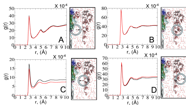
Fig. 6 RDFs depict the interactions between water–protein and water–glycan oxygen atoms in the closed (black) and open (red) states. Each RDF plot is accompanied by a schematic representation on the right side of the graph, denoting interfaces from left to right: protein, interfacial solvent, glycan, and bulk solvent. The positions of the radial circles where the RDF calculations were performed are shown. (A) RDF between water and protein oxygen atoms. (B) RDF between water and glycan oxygen atoms. (C) RDF between water and glycan oxygen atoms adjacent to the protein interface. (D) RDF between water and glycan oxygen atoms closer to the bulk solvent.
