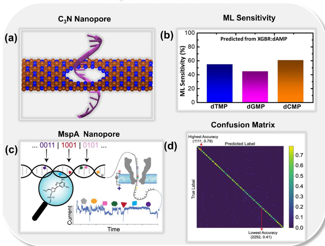
Fig. 6 (a) Schematic of C_3N nanopore 33 and (b) ML predicted sensitivity plot for DNA nucleotides dTMP, dGMP, and dCMP. 33 Reprinted with permission from ref. 33. Copyright 2023 American Chemical Society. (c) Schematic illustration of neural network-assisted MspA biological nanopore readout processing for different combinations and ordered sequences of natural and chemically modified nucleotides 34 and (d) confusion matrix with lowest and highest accuracy scores. 34 Reprinted with permission from ref. 34. Copyright 2022 American Chemical Society.
