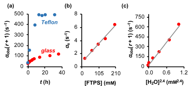
Fig. 3 Magnetisation transfer between TBAT and FTPS in THF (at 300 K). (a) An inherent increase of the magnetisation transfer rate with time in reactions conducted inside a dry and sealed glass NMR tube, and inside a dry Teflon insert (located within the NMR tube). (b) Under anhydrous, stabilised, non-acidic conditions, TBAT transfers fluoride to FTPS via parallel direct and dissociative mechanisms, with k_2^{\circ}c_{\text{FTPS}}/k_1 = 42 . \alpha_s/s^{-1} = 0.0273[\text{FTPS}/\text{mM}] + 0.656 , R^2 = 0.989 . (c) Exchange between the species is catalysed by water, with the order in water estimated as approximately 2. \alpha_{\text{obs}}(r + 1)/s^{-1} = 577[\text{H}_2\text{O}/\text{mM}]^{2.4} + 17.2 , R^2 = 0.989 .
