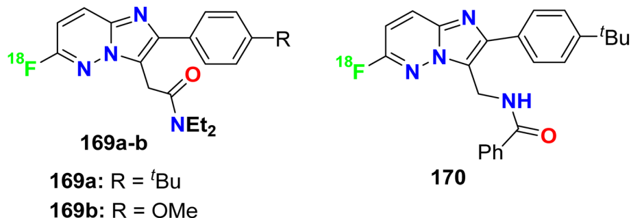
Fig. 86 Structure of fluorinated imidazo[1,2-a]pyridine heterocycles 169–170.
