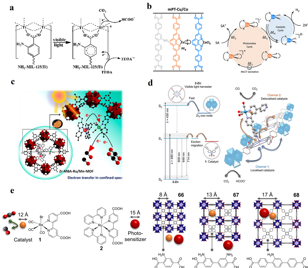
Fig. 6 Examples of different types of PS-CAT pairs in MOF-based photocatalysis: (a) type I ( \text{NH}_2\text{-BDC-Ti}_8 , linker-SBU) in \text{NH}_2\text{-MIL-125 (Ti)} MOF. Adapted with permission from ref. 65. Copyright 2012, WILEY-VCH Verlag GmbH & Co. (b) Type II ( [\text{Cu(PT)(dpe)}]\text{PF}_6\text{-[Co(PT)]}^{2+} , linker-linker) in \text{mPT-Cu/Co} MOF. Adapted with permission from ref. 75. Copyright 2020, the American Chemical Society. (c) Type III ( [\text{Ru(bpy)}_2(\text{MBA})]\text{-[Mn(MBA)(CO)}_3\text{Br)]} , SBU-SBU) in \text{Zr-MBA-Ru/Mn-MOF} (red balls: oxygen and black balls: carbon). Adapted with permission from ref. 79. Copyright 2023, the American Chemical Society. (d) Type IV (2-Zn-1 dyad) in Re-PCN hybrids (2-Zn: Zn-TCPP linker and 1: \text{fac-[ReBr(CO)}_3(\text{qtpy})] ). Reproduced with permission from ref. 82. Copyright 2022, the Royal Society of Chemistry. (e) Type V (encapsulated 1: [\text{ReBr(CO)}_3(4,4'\text{-dcbpy})] and 2: [\text{Ru(bpy)}_2(5,5'\text{-dcbpy})]\text{Cl}_2 ) in various assembly-controlling MOF topologies UiO (66, 67, 68). Adapted with permission from ref. 88. Copyright 2021, WILEY-VCH Verlag GmbH & Co.
