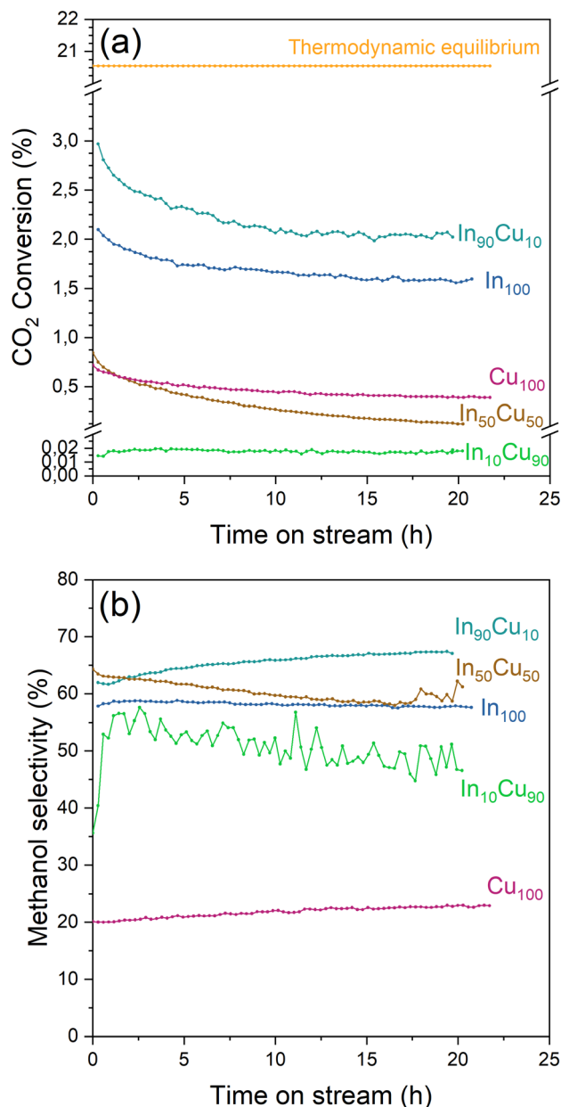
Fig. 8 (a) \text{CO}_2 conversion and (b) methanol selectivity of each catalyst during the stability test. Reaction conditions: 20 \text{NL h}^{-1} \text{g}_{\text{cat}}^{-1} , \text{H}_2/\text{CO}_2/\text{N}_2 = 15/5/1 molar ratio, 21 bar, 275 °C for 20 h.
