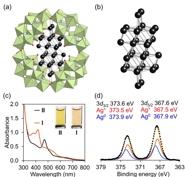
Fig. 2 (a) Crystal structure depicting the anion part of II . Green octahedra, \{WO_6\} ; purple tetrahedra, \{PO_4\} ; black spheres, Ag atoms; white spheres, O atoms. (b) Structure of an \{Ag_{30}\}^{18+} nanocluster in II . (c) UV-vis spectra of I and II in acetonitrile (10 \mu M, 1 cm quartz cell). (d) XPS spectrum in the Ag 3d region of II (black dots) and the sum of the curve-fitting analysis (orange line) obtained through the linear combination of Ag^0 (blue line) and Ag^+ (red line) with an area ratio of Ag^0/Ag^+ = 12/18 .
