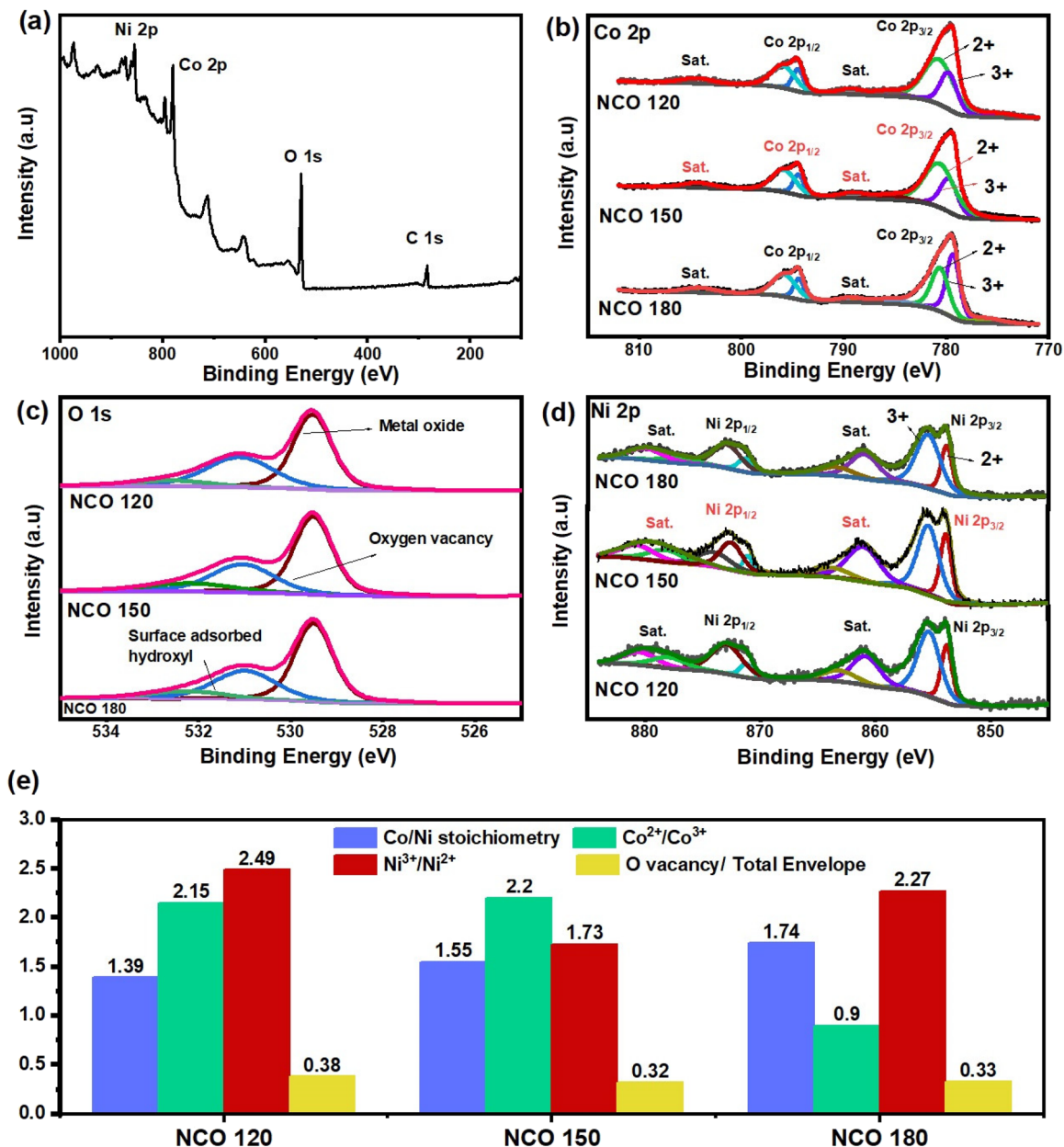
Fig. 3 XPS analysis: (a) survey spectrum, (b) Co 2p spectra, (c) O 1s spectra, (d) Ni 2p spectra of as-synthesized NiCo 2 O 4 catalysts on Ni foam, and (e) extrapolated co-relations via peak area analysis.
