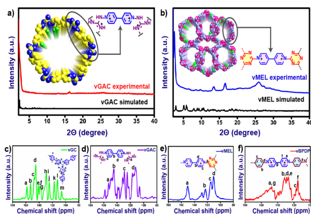
Fig. 3 Comparison of experimental PXRD pattern with the simulated powder pattern of (a) vGAC and (b) vMEL. Solid-state ^{13}\text{C} CP-MAS NMR spectra of (c) vGC, (d) vGAC, (e) vMEL and (f) vBPDP.
