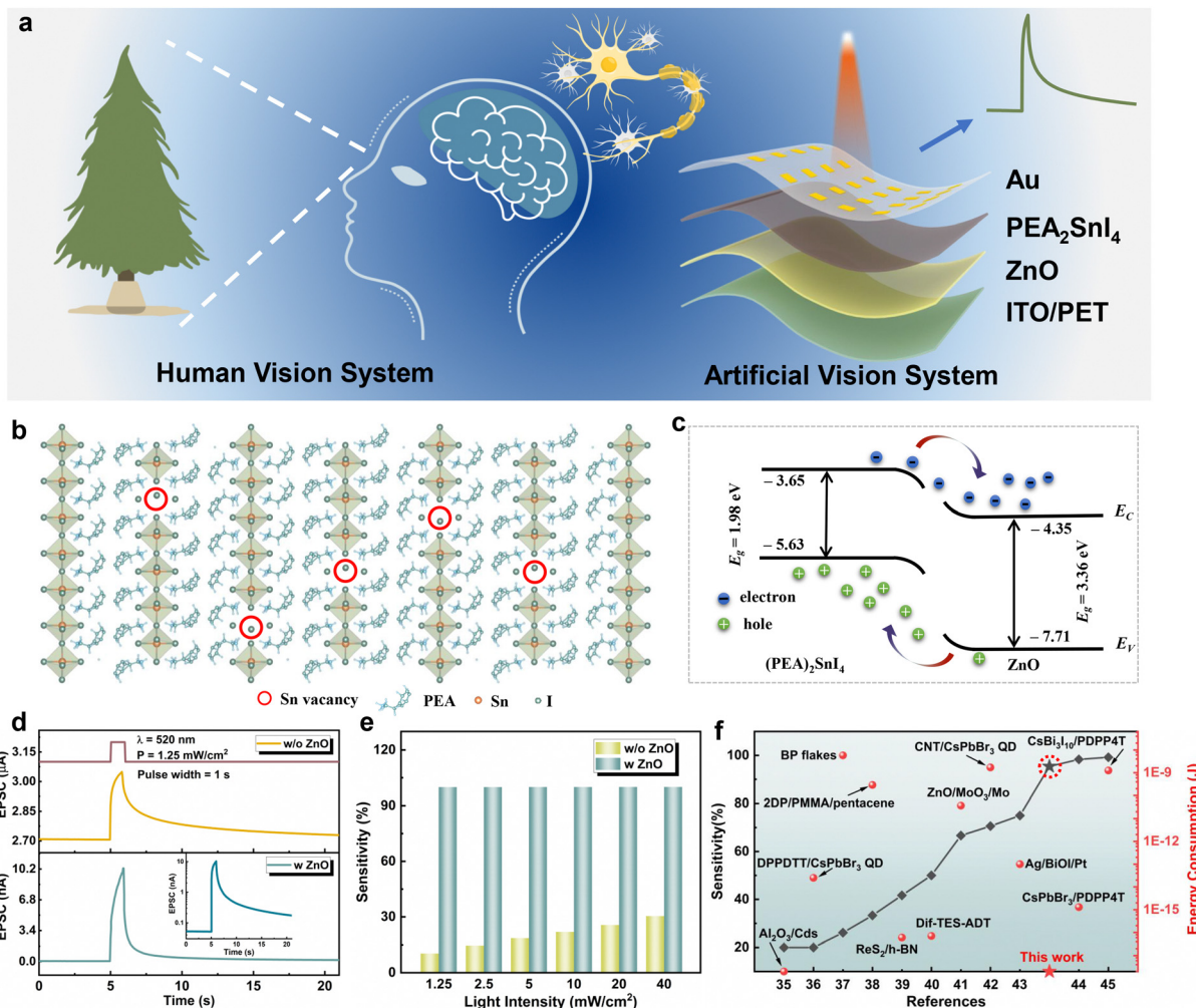
Fig. 1 (a) Schematic structure of the bionic human vision system and the proposed optoelectronic synaptic device structure. (b) Schematic illustration of Sn vacancy formation in \text{PEA}_2\text{SnI}_4 perovskite. (c) Energy band diagram of the \text{PEA}_2\text{SnI}_4/\text{ZnO} heterojunction under illumination without power supply. (d) EPSC behavior of the \text{Au}/\text{PEA}_2\text{SnI}_4/\text{ITO} and \text{Au}/\text{PEA}_2\text{SnI}_4/\text{ZnO}/\text{ITO} device triggered by a light pulse (inset shows the graph of the corresponding logarithm). (e) S versus light intensity of the two types of devices. (f) Comparison of customized sensitivity and energy consumption from previously reported devices. 35–45
