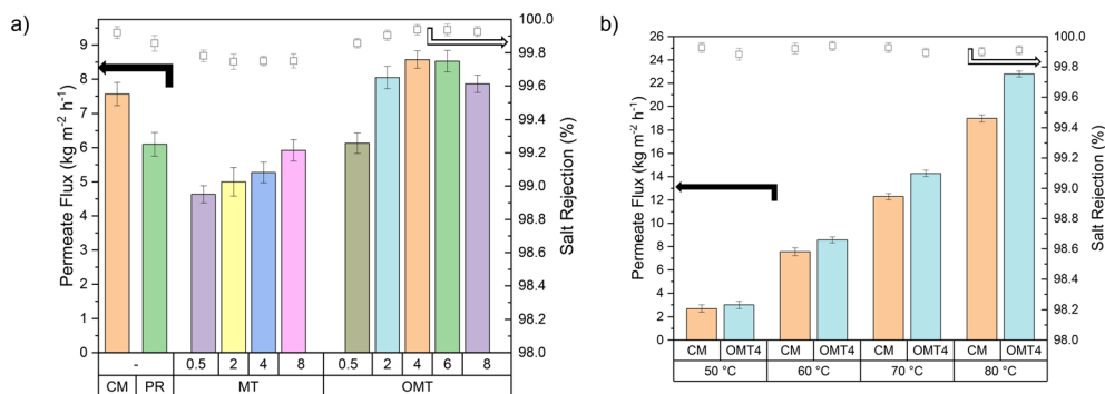
Fig. 6 Average total permeate flux and salt rejection of the prepared PVDF-clay membranes at a) 60 °C and at b) different feed temperatures for commercial PVDF and the OMT 4 wt% membranes. Columns: permeate flux (kg m -2 h -1 ), and square symbols □: salt rejection (%). Error bars represent standard deviations from three samples.
