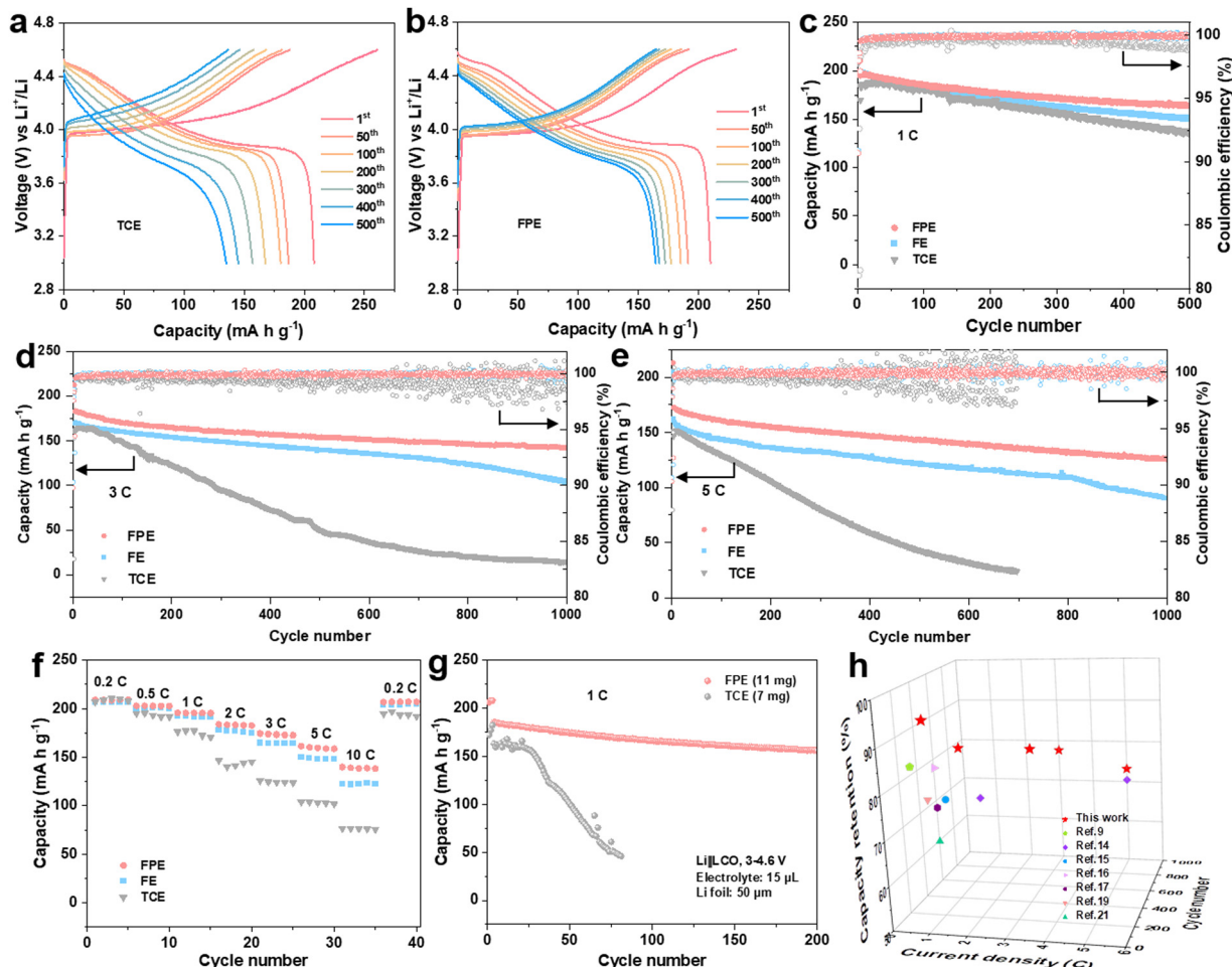
Fig. 2 Electrochemical performance of a 4.6 V LCO cathode at 3–4.6 V (vs. Li + /Li) in FPE. (a) and (b) Charge–discharge voltage profiles of Li||LCO cell at 1C ( 1\text{C} = 274\text{ mA g}^{-1} ) in (a) TCE and (b) FPE. (c)–(e) Cycling stabilities at (c) 1C, (d) 3C fast charging/discharging, and (e) 5C superfast charging/discharging performance of Li||LCO cells in three electrolytes. (f) Rate capability of Li||LCO cells in three electrolytes. (g) High-voltage Li||LCO full cells in practical conditions (thick cathode of 10\text{ mg cm}^{-2} , thin Li anode of 50\text{ }\mu\text{m} , and lean electrolyte of 15\text{ }\mu\text{L} ) in TCE and FPE. (h) Comparison of cycling stability and fast-charging performance of 4.6 V LCO cathodes with reported LCO works in advanced electrolytes.
