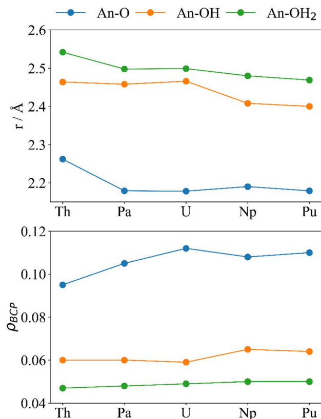
Fig. 7 Optimised distances r (Å, upper) and \rho_{\text{BCP}} (a.u., lower) for \{(\text{An}(\text{H}_2\text{O})_5)(\text{Na}(\text{H}_2\text{O})_2)_5\text{Fe}_{13}\text{O}_{28}\text{H}_{12}\}^{4+} (calculated at the PBE0/Def2TZVP/SARC-DKH2 level).
