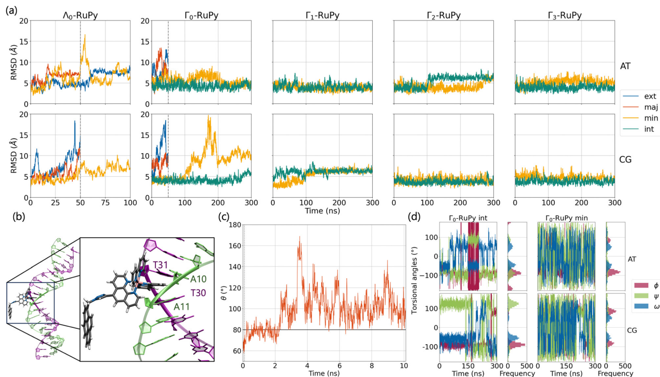
Fig. 8 (a) RMSD values of production run trajectories computed against the starting structures for \Lambda_0 -RuPy and \Gamma_0 -RuPy with i = 0, 1, 2, 3 structures initially placed interacting externally (ext), in the major groove pocket (maj), in the minor groove pocket (min) or intercalated between two nucleobase pairs (int) of both poly(dA)poly(dT) (top) and poly(dC)poly(dG) (bottom) DNA double strands. (b) Partial intercalation of a bpy ligand of \Gamma_0 -RuPy between the nucleobase pairs A10-T31 and A11-T30. (c) Time evolution of angle \theta in the heating and equilibration stages of the simulation when \Lambda_0 -RuPy is initially placed in the major groove pocket of poly(dA)poly(dT) DNA double strand. The horizontal line at 80 indicates the threshold for distinguishing between \Lambda -shaped geometry ( \theta < 80 ) and \Gamma -shaped geometry ( \theta > 80 ). (d) Time evolution and histogram of \phi , \psi and \omega torsional angles along the production runs for \Gamma_0 -RuPy initially placed in intercalated between two nucleobase pairs (int) and in the minor groove pocket (min) of both poly(dA)poly(dT) (top) and poly(dC)poly(dG) (bottom) DNA double strands.
