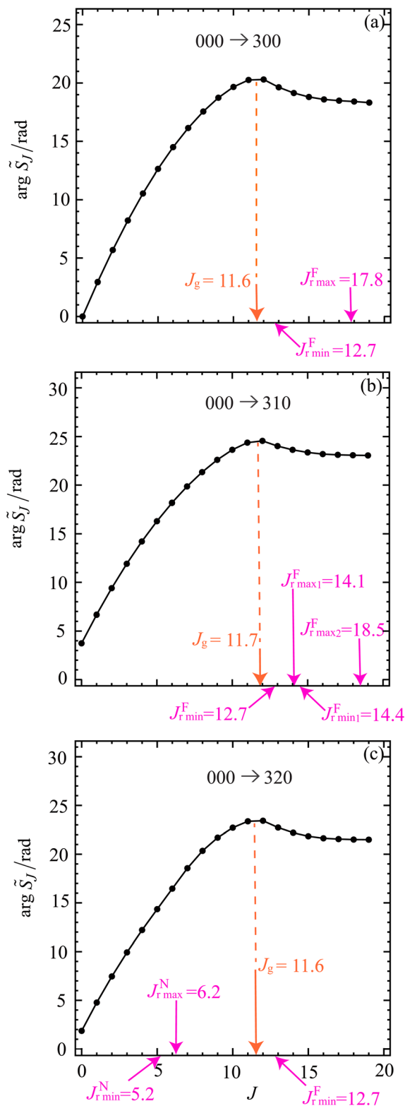
Fig. 2 Plots of \arg \tilde{S}_J / \text{rad} versus J at E_{\text{trans}} = 62.09 \text{ meV} . The black solid circles are the numerical S matrix data, \{\arg \tilde{S}_J / \text{rad}\} , at integer values of J , which have been joined by straight lines. The dashed orange lines and orange arrow indicates the value of the glory angular momentum variable, J_g . The pink arrows indicate the values of the nearside (N) and farside (F) rainbow angular momentum variable. The notation and values of J_g , and the rainbow angular momenta, are taken from Fig. 6. The transitions are: (a) 000 \rightarrow 300 , (b) 000 \rightarrow 310 , (c) 000 \rightarrow 320 .
