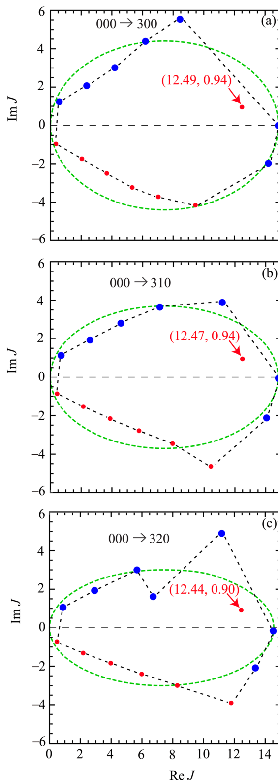
Fig. 3 Plots of the CAM J plane at E_{\text{trans}} = 62.09 \text{ meV} using Thiele rational interpolation for \{\tilde{S}_J\} with integer values of J as input. There are 7 poles (red) and 7 zeros (blue) of \tilde{S}_J . The inside of the green-dashed ellipse, or the black-dashed polygon, shows approximately the region of stability for \tilde{S}_J . There is one stable Regge pole in the first quadrant of the CAM plane, accompanied by boundary poles and zeros. The transitions are: (a) 000 \rightarrow 300 , (b) 000 \rightarrow 310 , (c) 000 \rightarrow 320 .
