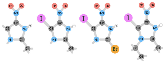
Fig. 1 Schematic picture of the studied protonated molecules. From left to right: \text{NimH}^+ , \text{INimH}^+ , \text{BrNimH}^+ , and \text{EtNimH}^+ .
