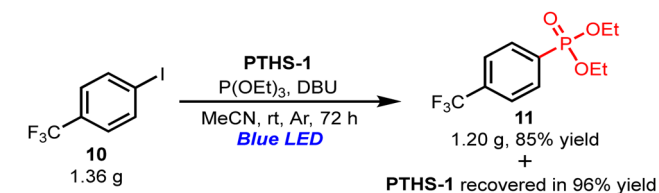
Scheme 2 Gram-scale photoredox cross-coupling reaction of 4-iodo-1-(trifluoromethyl)benzene with triethylphosphite. The reaction was carried out with 10 (5.0 mmol), triethylphosphite (15.0 mmol), DBU (10.0 mmol), and PTHS-1 (10 mol%) in MeCN at room temperature under an Ar atmosphere and blue LED irradiation ( \lambda_{\text{max}} = 425 \text{ nm} , 18 W).
