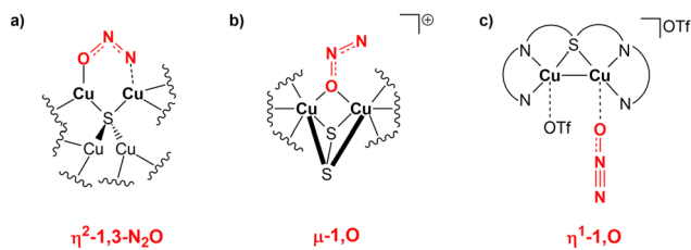
Scheme 7 (a) Proposed \eta^2-1,3-N_2O binding mode at the two copper centres of the nitrous oxide reductase enzyme. (b) and (c) Observed N_2O binding modes over copper centres in biomimetic dicopper compounds.
