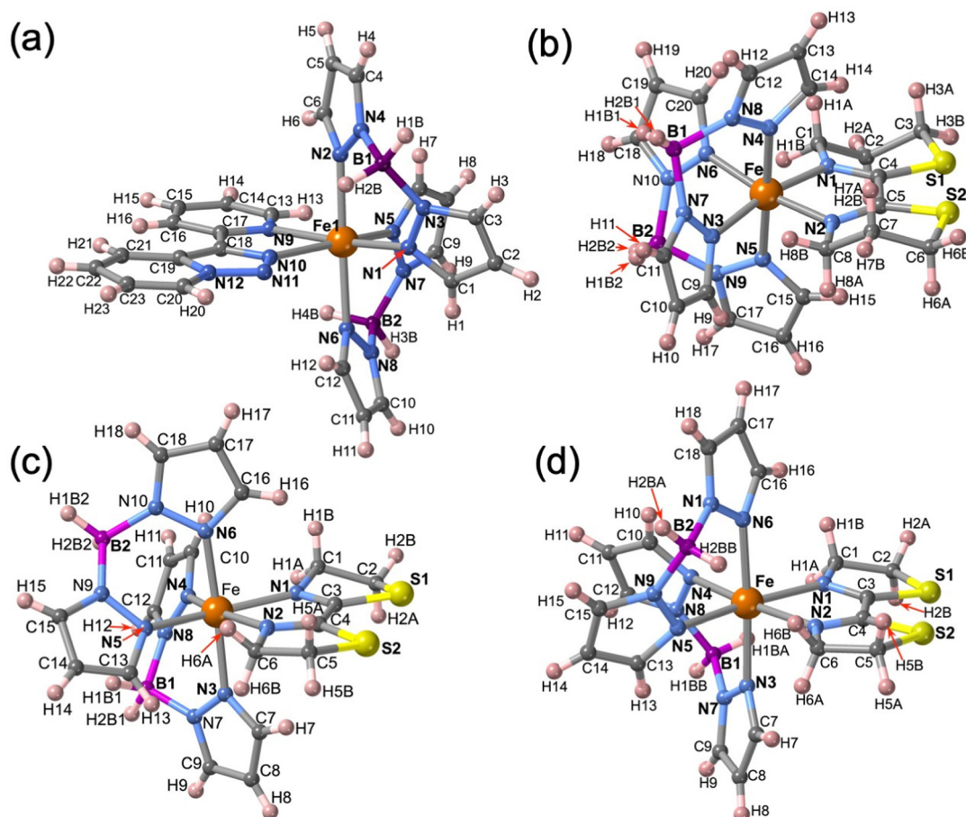
Fig. 2 Molecular unit of 1-CH 3 CN , 2 , 3 \cdot 1/2\text{CH}_2\text{Cl}_2 and 3 , showing the atom numbering. Only one of the two Fe II centres (Fe1) is shown in 1-CH 3 CN , for Fe2 (see Fig. S3, ESI†).
